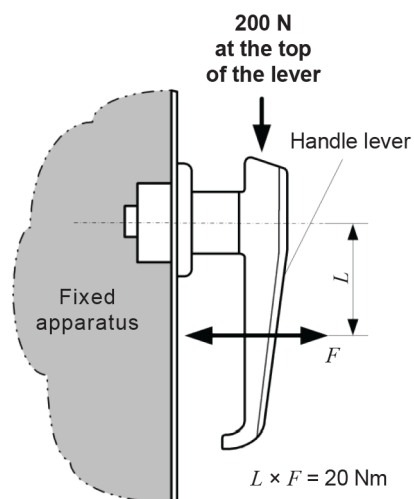
b) Handle, lever type
