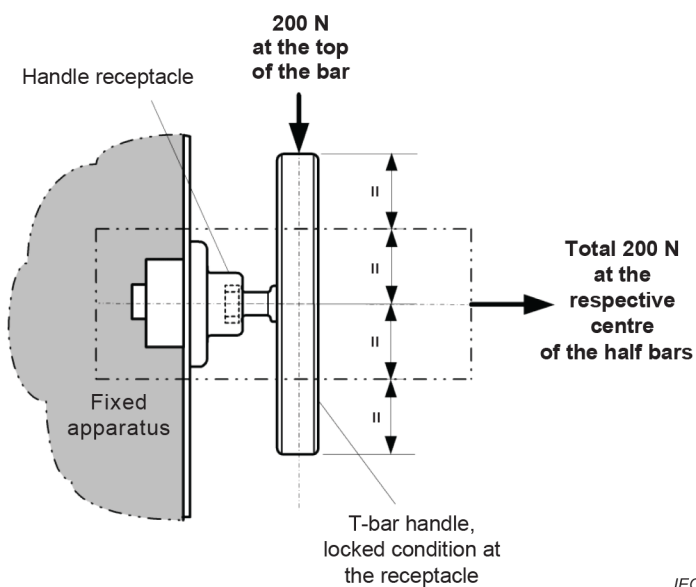
c) Handle, T-bar type
