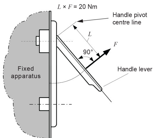
a) Handle, flat lever type
